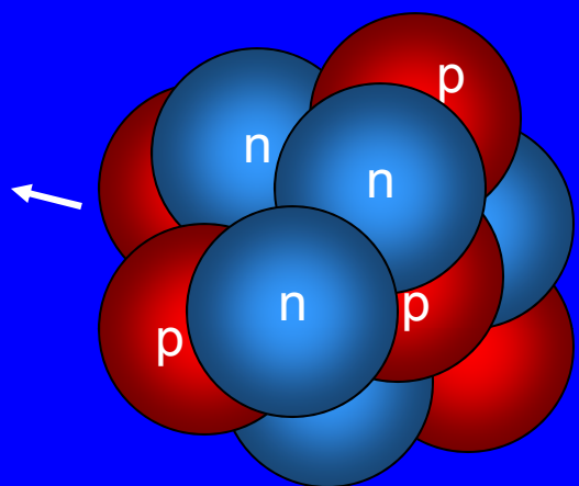
Decay Product
