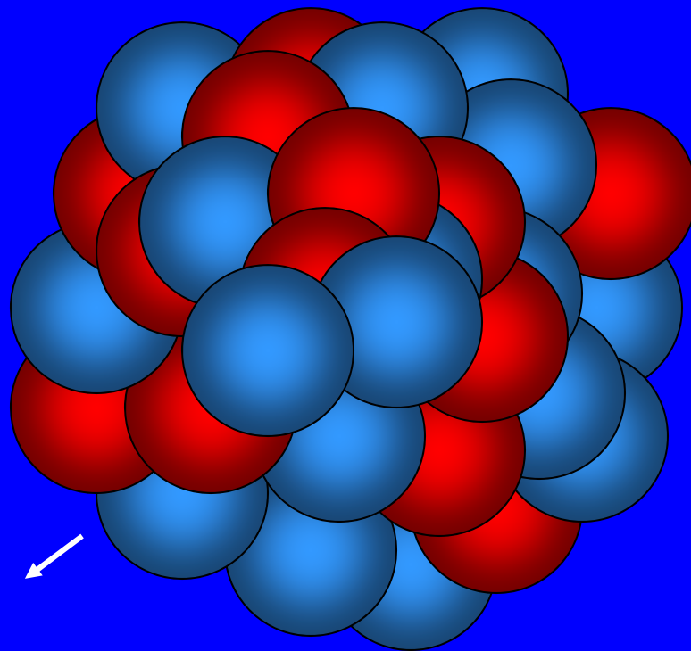
Decay Product
