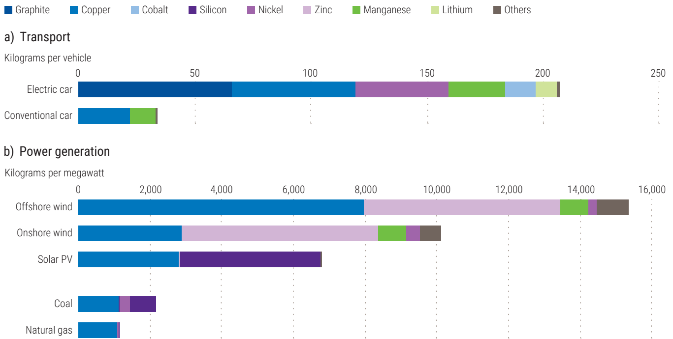
Figure II.1 Critical minerals used in selected clean energy technologies and traditional energy technologies
