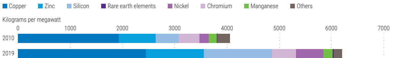
Figure II.2 Average critical mineral intensity of new power generation capacity
